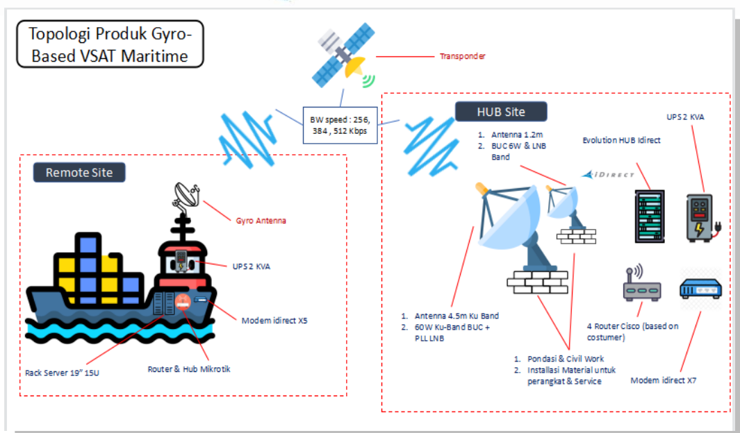
Gambar-1: Topologi Produk Gyro-Based VSAT Maritime
